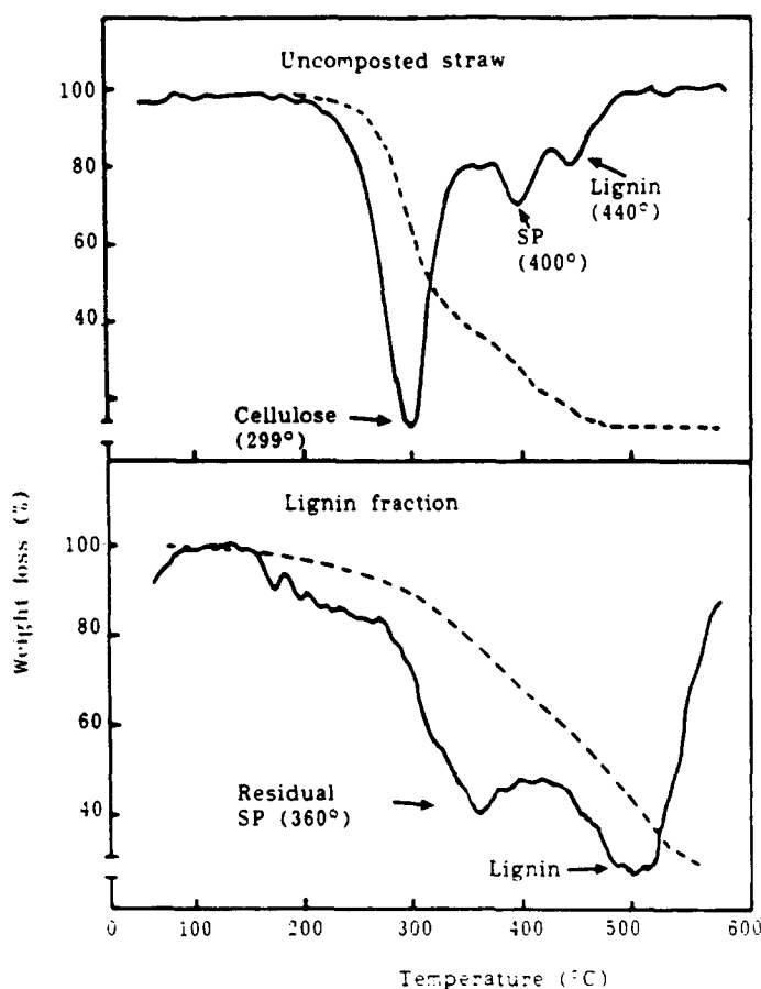
Fig. 3. Thermograms of uncomposted wheat straw and lignin separated from the straw showing the TG weight loss (--) and DTG profiles (—) of structural polysaccharides (SP), cellulose and lignin present in the samples.
