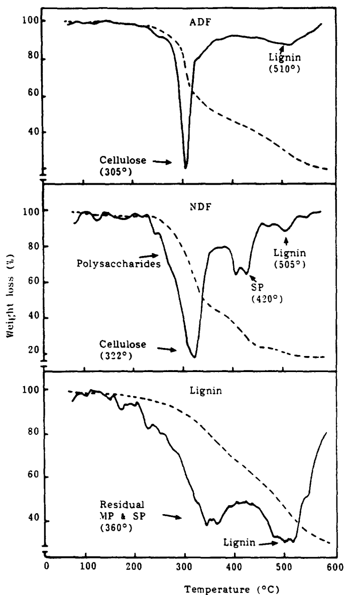
Fig. 1. Thermograms of ADF, NDF and lignin fractions separated from the compost samples showing the TG weight loss (---) and DTG profiles (—) of microbial polysaccharides (MP), structural polysaccharides (SP), cellulose and lignin present in the samples.
