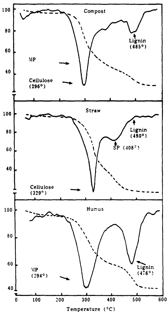
Fig. 2. Thermograms of compost and its fractions humus and straw obtained by ultrasonic treatment showing the TG weight loss (--) and DTG profiles (—) of microbial polysaccharides (MP), structural polysaccharides (SP), cellulose and lignin present in the samples.
